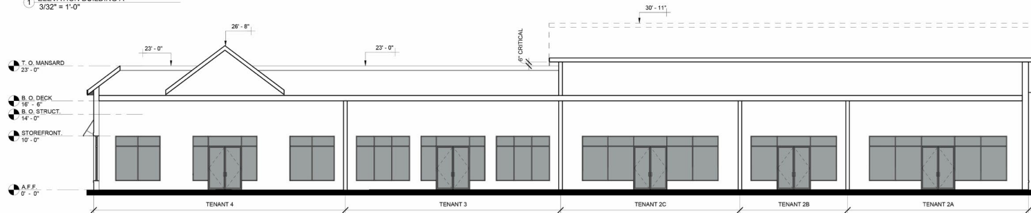
② SCHEMATIC BUILDING A SECTION 1/8" = 1'-0"
